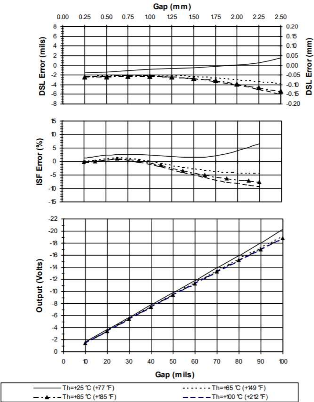
Figure 7: Typical 3300 XL 8mm 9m Proximitor Sensor with 8m Extension Cable at T_h (Probe is at 25 ^{\circ}\text{C} )
