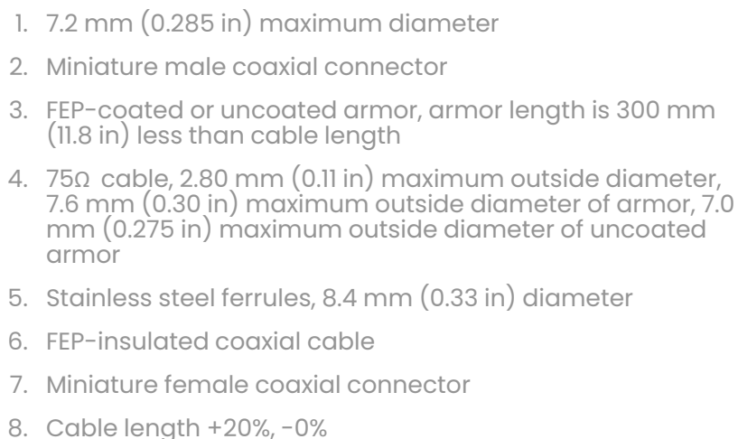
Figure 6: 3300 NSv Extension Cable
